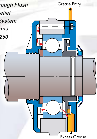
TECO Through Flush Grease Relief Bearing System with Brass Dust Flinger D280-355
