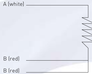
“3 wire” RTD circuit
