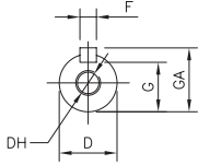
SHAFT DETAIL
