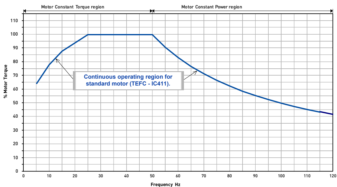
Typical Motor Loadability Curves For VSD Duty
